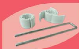
Core Adapters
