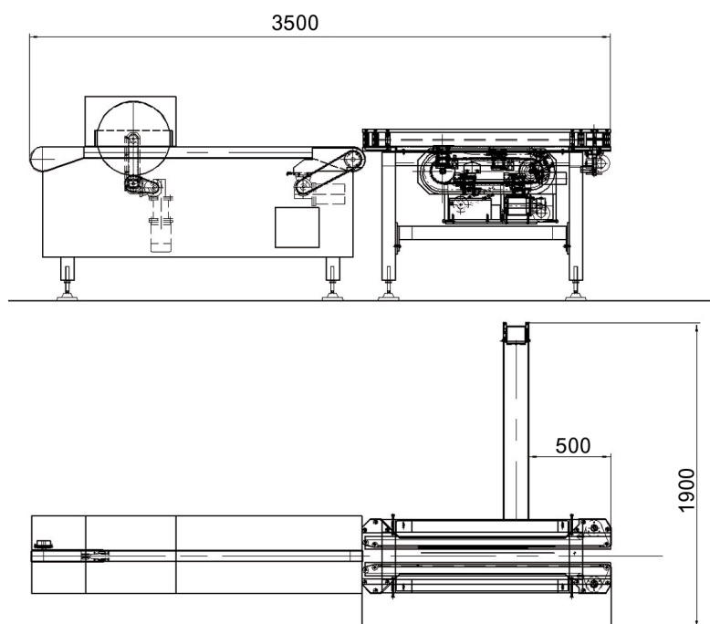
self standing lid applicator
