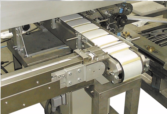
Plastic lid applicator onto the film
